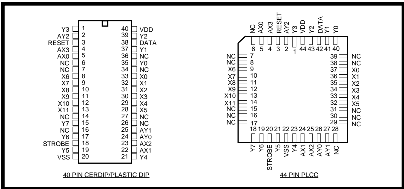
Figure 2 - Pin Connections
